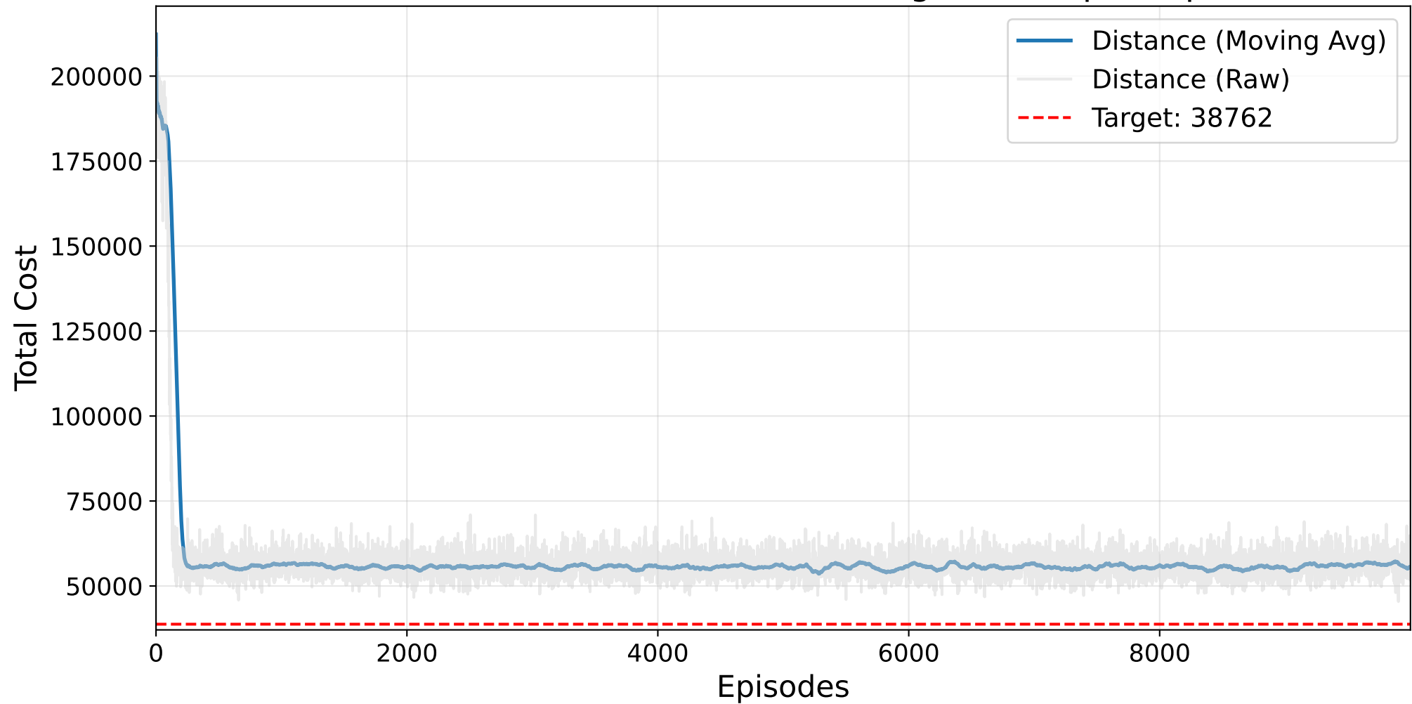
Final Masked AutoRL-SOP Training - kro124p.1.sop
